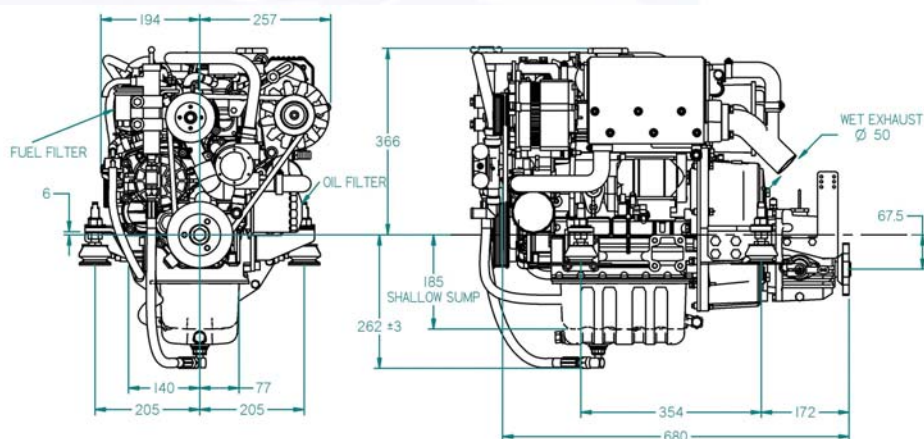
Engine shown with optional Down Angle Gearbox
